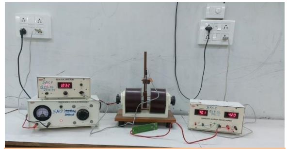
18. Hall Effect Measurement Setup
