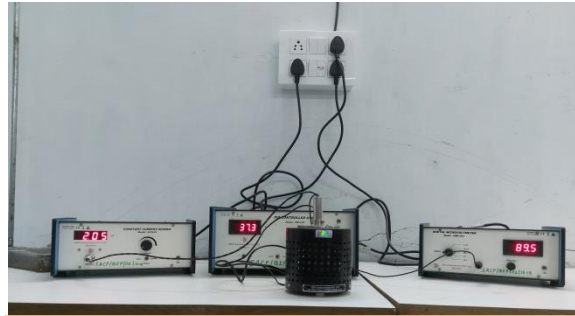
21. Four Probe Method Setup
