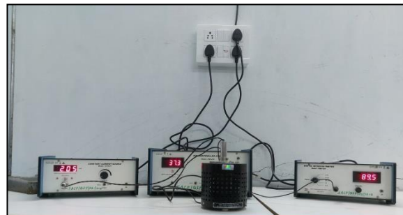
Four Probe Method Setup
